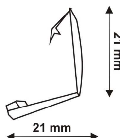
LATERAL SIDE
